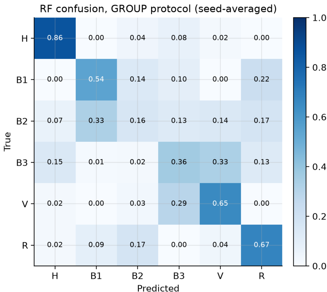
Figure 7. Seed-averaged confusion matrix of the Random Forest under the GROUP protocol. Healthy (H) and broken-rotor-bar (R) states are the most separable; the lubrication-severity states (B1, B2) are the most confused.
